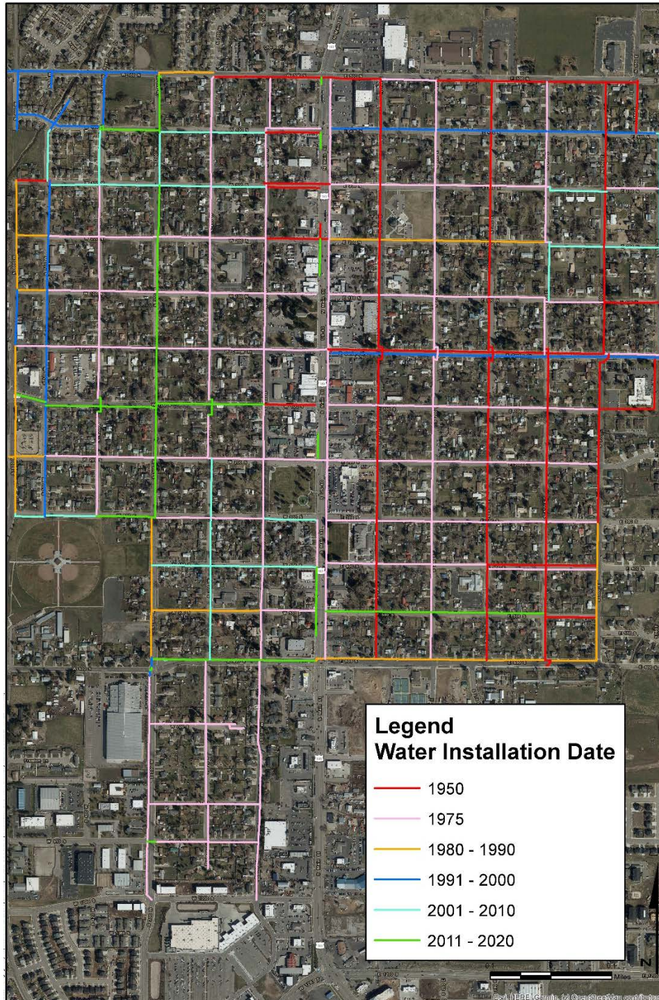
Figure 3: Water Pipe Installation Dates
